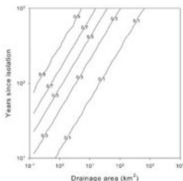
Figure 6. Curves estimating the probability of extinction for isolated populations of resident (i.e., nonmigratory) fish as a function of the drainage basin size and time since the basin was isolated, based on analyses of postglacial losses by Hugueny et al. 100 These estimates are very approximate, and probably underestimate extinction rates in modern drainage basins that are heavily affected by human activities, but illustrates the strong dependence of species losses in isolated basins on the size of the basin and time since isolation.
